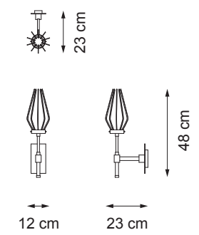
Item D07 1 light wall lamp (E14 40W max)
