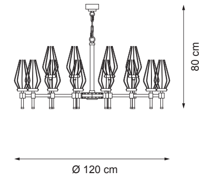
Item D01 24 lights chandelier (E14 40W max)
