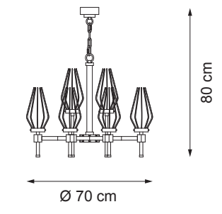
Item D03 16 lights chandelier (E14 40W max)
