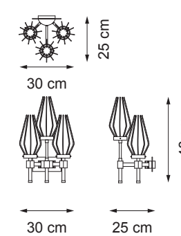
Item D05 3 lights wall lamp (E14 40W max)
