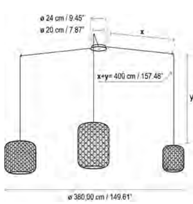
Nans S/3L INDOOR IP-20
