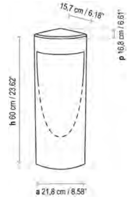
Moai B/60 IP66
