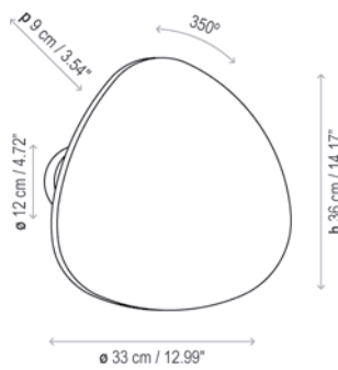
Tria 05 IP66
