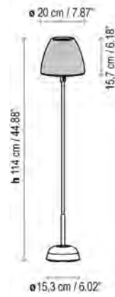
Atticus P/114/R IP-66
