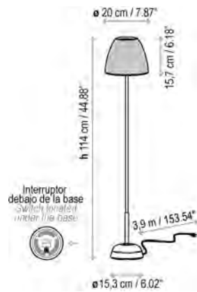
Atticus P/114 IP-66
