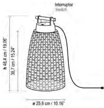
Nans Portable M/49 IP-65
