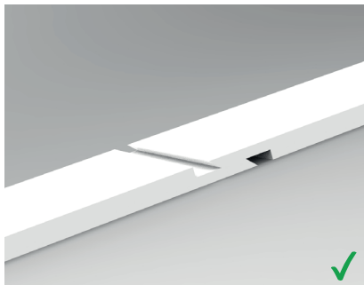
Überlappung 5 mm
