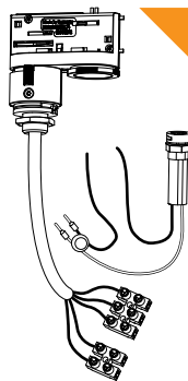
ERCO OEM DALI adapter
