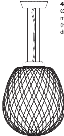
4363.. Ø 30 x 36 + 250 cm max 1 x 116W E27 (HA, FL, Led) dimnable
