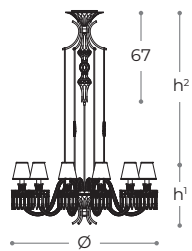
MARGOT . 461/12C . design by Roberta Vitadello Lampada a sospensione - Chandelier . p. 24
