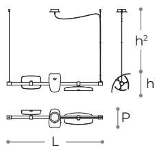
AXI . T1805/SO . design by Patrick Jouin ID Lampada a sospensione - Suspension lamp . p. 36
