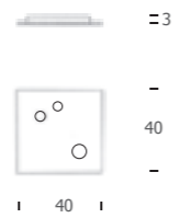
DES•AGN 50.3 p/pl round/square Wall/ceiling lamp in steel cm 40X40X3 3 led COB 10W - max 250mA 3300 Lm emitted 3000°K - CRI>85 Power supply included •Dimmable on request
